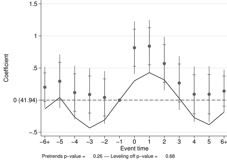
Figure 4: Least wiggly path through the confidence region
